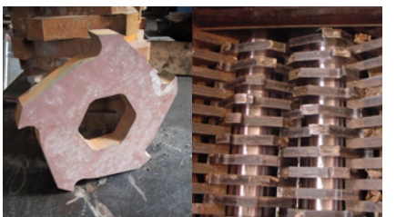
4. SHREDDERS Hardox 500, 550 or 600. Hardox can also be used in shredders. The specific steel grade depends on the sorted material and the frequency of tough, hard-crushed objects in the machine. The high toughness of Hardox steels provides shredders with a substantially higher resistance against cracking and cleavages.
